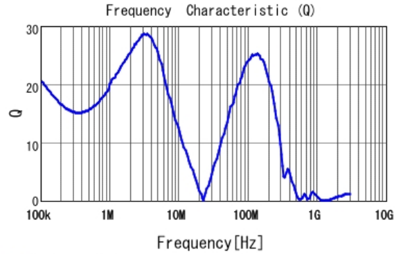
■ 1267AY-150M Q
