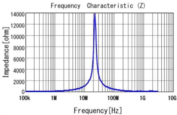
■ 1267AY-150M |Z|
