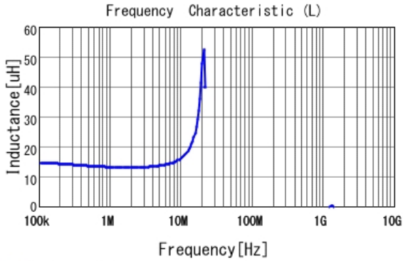
■ 1267AY-150M L
